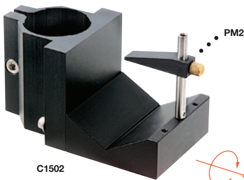
±10° Manual Pitch Adjustment
