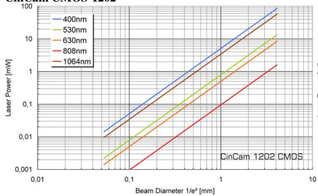
CinCam CMOS-1202
