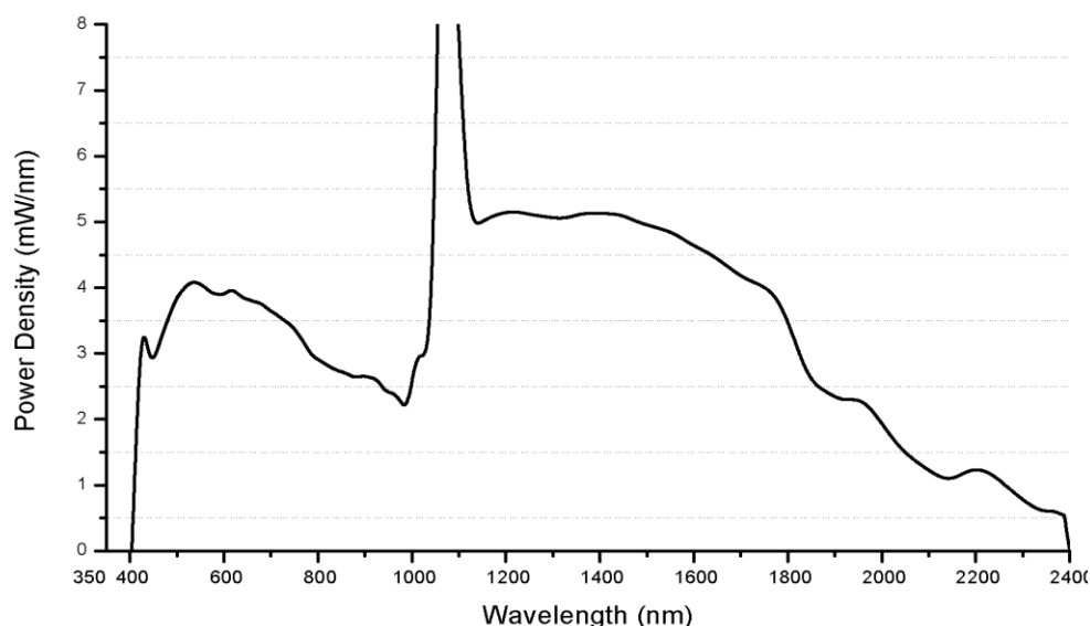
8W SC Pro Typical Spectrum (4MHz)
